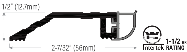
DS222AV Extruded aluminum mill finish with vinyl insert, grey DS222DV Bronze anodized
