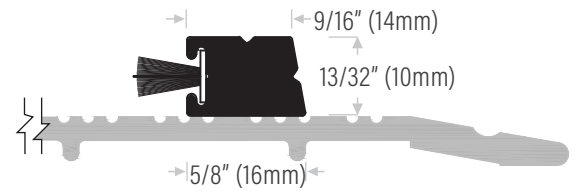
DS176AP Extruded aluminum mill finish with pile insert, grey, not rated . Threshold not included, order separately
