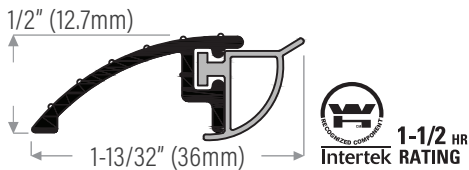
DS121AV Extruded aluminum mill finish with vinyl insert, grey DS121AVBL Mill finish with vinyl insert, black DS121WV White with grey insert DS121BVBL Brown with black insert
