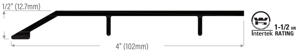
DS444AS Extruded aluminum mill finish
