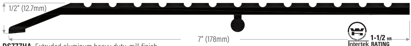
DS777HA Extruded aluminum heavy duty, mill finish
