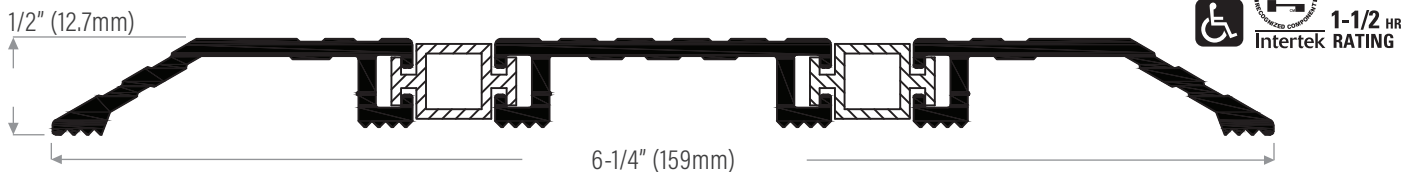
DS603TBA Extruded aluminum mill finish with 2 thermal breaks
