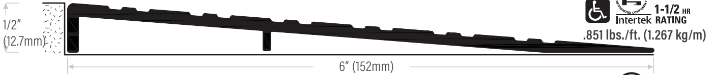
DS606A Extruded aluminum mill finish
