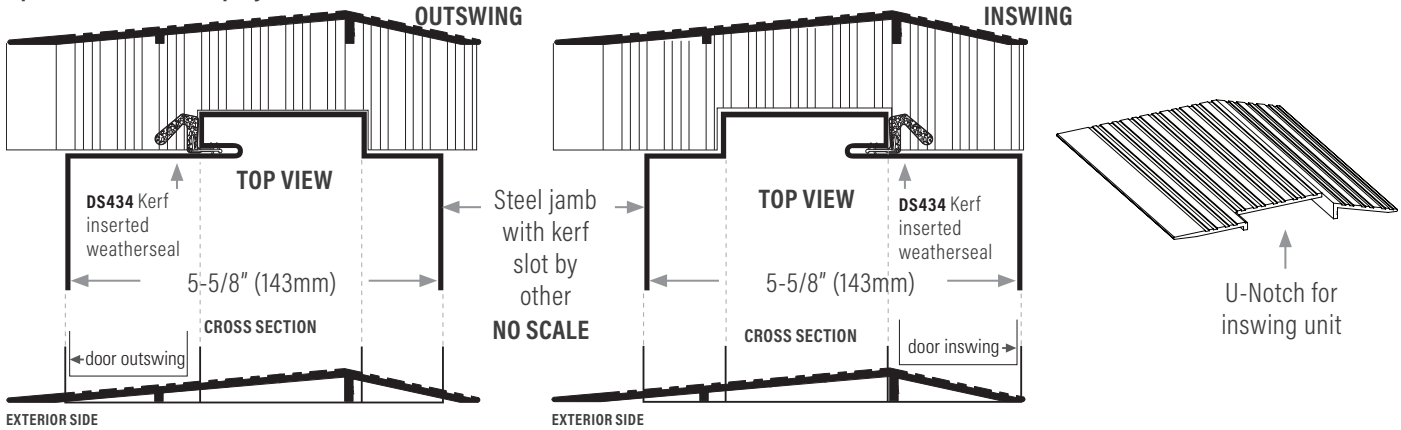
DS707A Extruded aluminum mill finish
