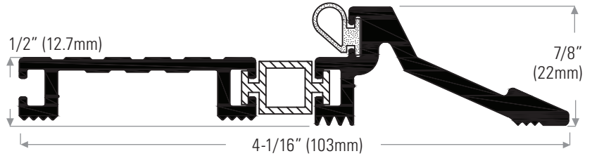
DS276TBAT Extruded aluminum mill finish with vinyl thermal break insert & TPE (T) insert
