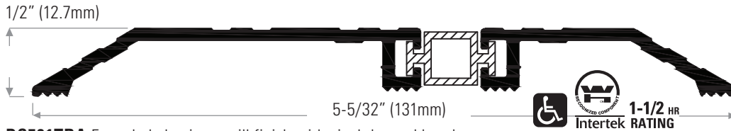
DS501TBA Extruded aluminum mill finish with vinyl thermal break
