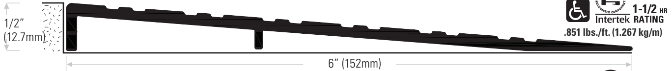
DS606A Extruded aluminum mill finish
