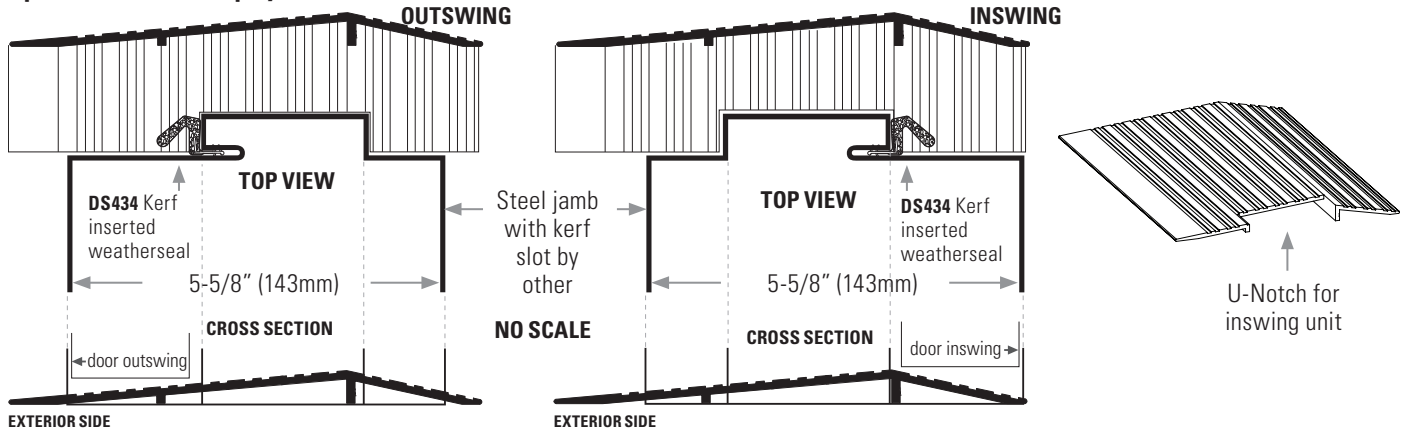
DS707A Extruded aluminum mill finish
