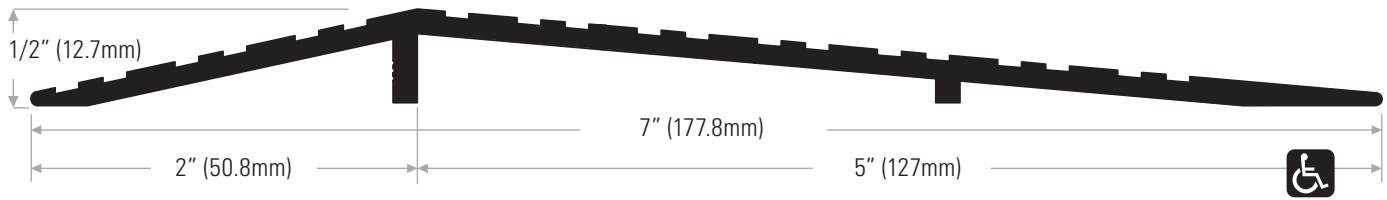
DS707A Extruded aluminum mill finish
