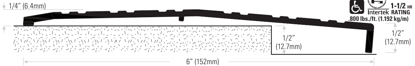
DS605A Extruded aluminum mill finish
