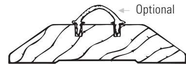
DS3530AKV Oak threshold with vinyl insert, tan
