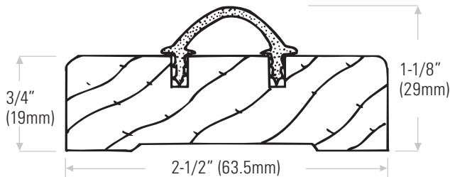
DS2230AKV Oak threshold with vinyl insert, tan
