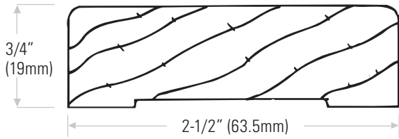
DS2230AK Oak threshold
