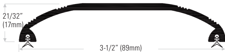
DS218A Extruded aluminum mill finish with vinyl feet
