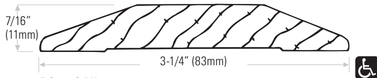
DS3510AK Oak threshold
