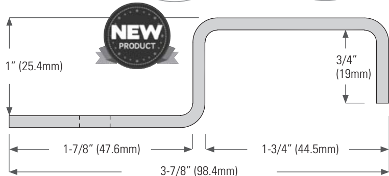
DS187PS Steel prime coated, standard. Lengths available 84" (2134mm), 96" (2438mm) & 120" (3048mm)
