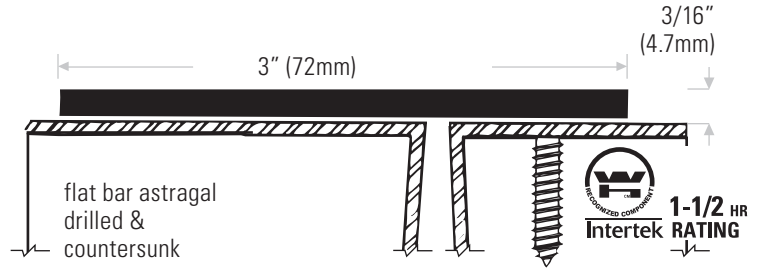
DS188-3PS Flat bar, steel prime coated 3" (76mm) wide
