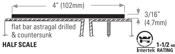
DS188-4PS Flat bar, steel prime coated 4" (102mm) wide
