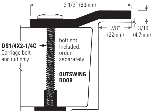
DS179PS Steel prime coated DS179SS Stainless steel satin finish. Three week delivery. Intertek 1-1/2 HR RATING
