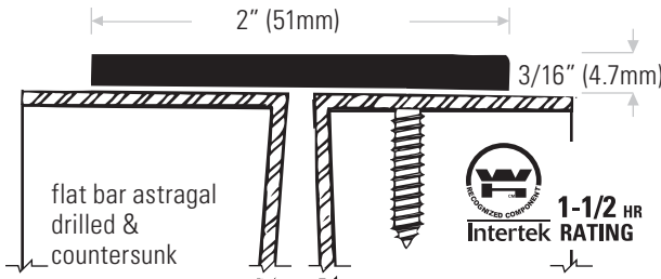
DS188-2PS Flat bar, steel prime coated 2" (51mm) wide
