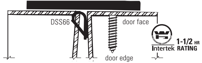
DSS66 Used in conjunction with flat bar astragal
