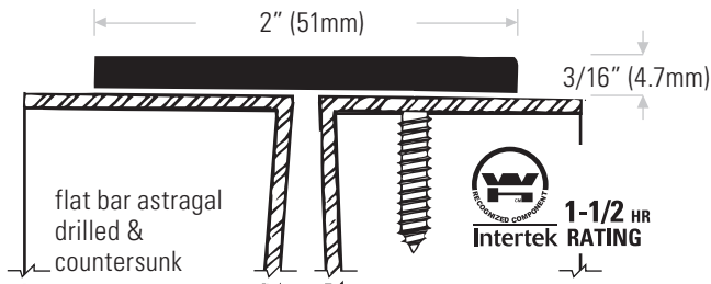
DS184SSATIN Flat bar, stainless steel Lengths available: 84" (2134mm), 96" (2438mm), 144" (3658mm)
