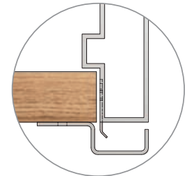
DS186PS Steel prime coated, custom. Lengths available 84" (2134mm), 96" (2438mm) & 120" (3048mm)
